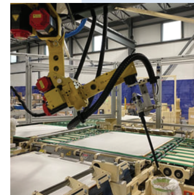
Adhesive Dispensing
